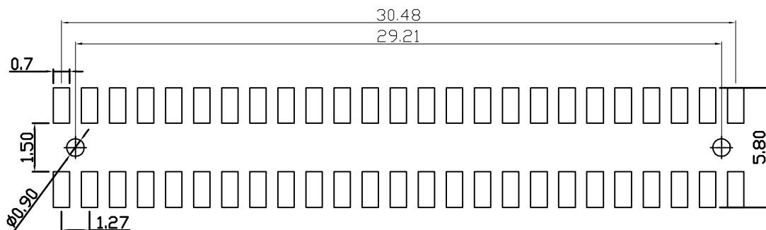
PCB Layout
